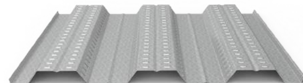
Tôn sàn 3 sóng H75 - W865 H75 - W865 3 square decking panel
